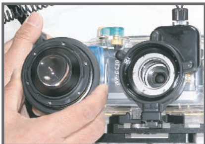
AD Mount Series Lens can be easily installed into 'AD Mount Base' and 28AD Mount Series Lens can be easily installed on '28AD Mount Base' / '28AD Port'. It is free from abrupt dropping off. You can have free choice among Wide Conversion Lens, Fish-eye Lens or Close-up Lens depending on your subjects and easily exchange lens underwater.
