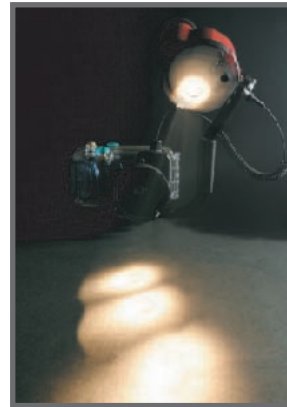
Simple strobe positioning depending on distance to subject by swinging D-2000 on the arm. That's it. You can check if the axis of strobe situate in right position with Focus Light. Focus light never expose on image since it automatically turns off during exposure.
